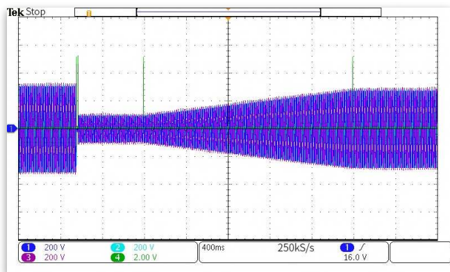
Three-Phase Low Voltage Ride Through
