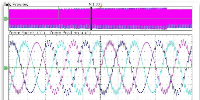
Inter-harmonic Sweep
