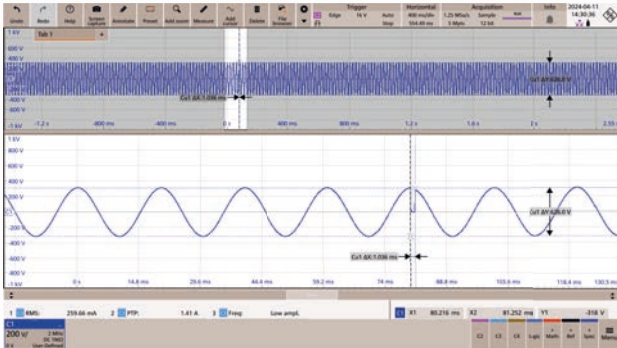
1ms interruption
