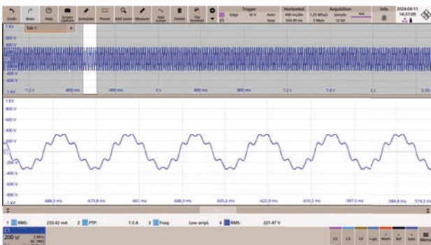
Harmonic injection
