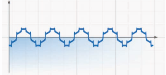
IEC61000-4-13 Odd harmonics that are not multiples of 3 @Class3/50Hz
