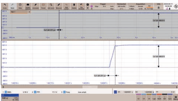
Dynamic response time : 251 \mu s
